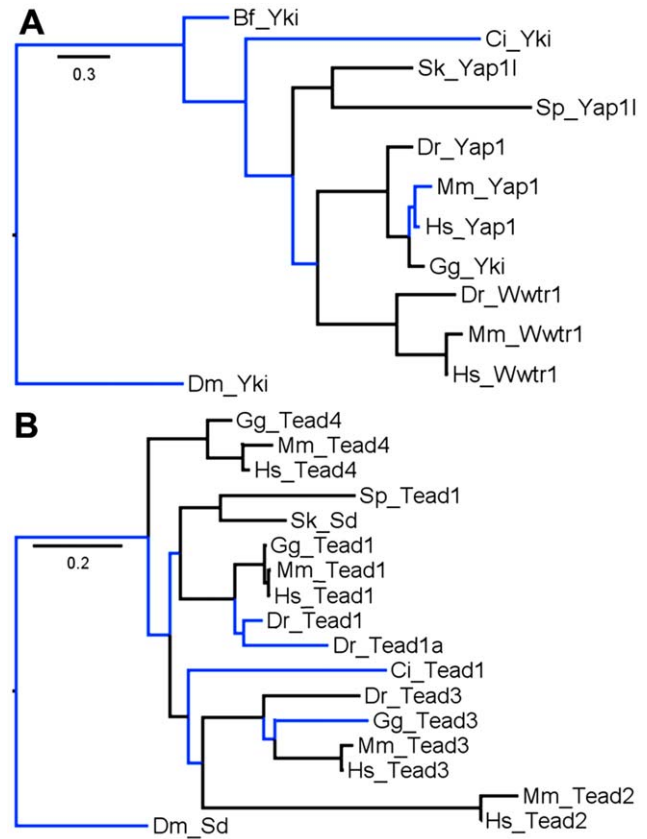
Figure 4. Yorkie/Yap/Taz and Scalloped/Tead Maximum Likelihood trees. A) Yorkie/Yap/Taz (Taz is formally known as Wwtr1) vertebrate topology matches the species tree. Among invertebrates there is strong pairing of the echinoderm and hemichordate but weak connections of this pair to cephalochordates, urochordates and vertebrates in relationships that deviate from the species tree. The Bayesian tree (Figure S1E) shows one difference - the urochordate has switched places with the cephalochordate exaggerating the deviation from the species tree. B) Scalloped/Tead vertebrate topology matches the species tree. Among invertebrates, the tree clusters the hemichordate and echinoderm with vertebrate Tead1 without the urochordate and clusters the urochordate with vertebrate Tead3, both are deviations from the species tree. The Bayesian tree (Figure S1F) shows one difference - the echinoderm and hemichordate move away from vertebrate Tead1 as outliers, an arrangement that is a slightly better match to the species tree. doi:10.1371/journal.pone.0051599.g004
