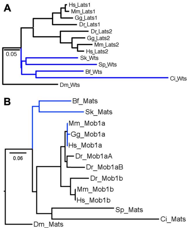
Figure 3. Warts/Lats and Mats/Mob Maximum Likelihood trees. A) Warts/Lats vertebrate topology matches the species tree. Among invertebrates, these proteins should be sequentially joined to the vertebrate cluster and thus this part of the Warts/Lats tree deviates from the species tree. The Bayesian tree (Figure S1C) shows one difference - rather than the hemichordate and echinoderm clustering together they are sequentially clustered with the large urochordate, cephalochordate and vertebrate group, an arrangement that better matches the species tree. B) Mats/Mob vertebrate topology matches the species tree except for difficulty resolving human, mouse and chicken Mob1a. Among invertebrates a cluster of the echinoderm and urochordate sequences is attached to the vertebrate cluster with the hemichordate and cephalochordates as outliers. The association of urochordates with vertebrates matches the species tree but the inclusion of echinoderms without hemichordates and cephalochordates does not. The Bayesian tree (Figure S1D) shows one difference - the urochordate switches places with the hemichordate leading to an arrangement that better matches the species tree but with no confidence. doi:10.1371/journal.pone.0051599.g003
