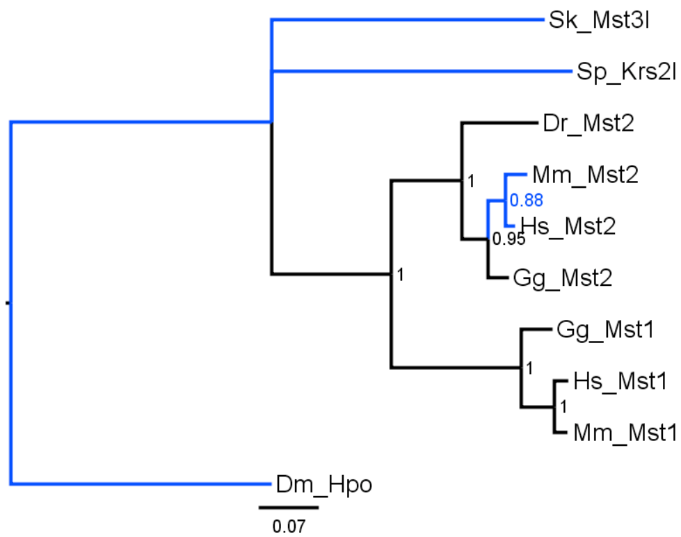
Fig. S1A. Hippo/Mst Bayesian tree
