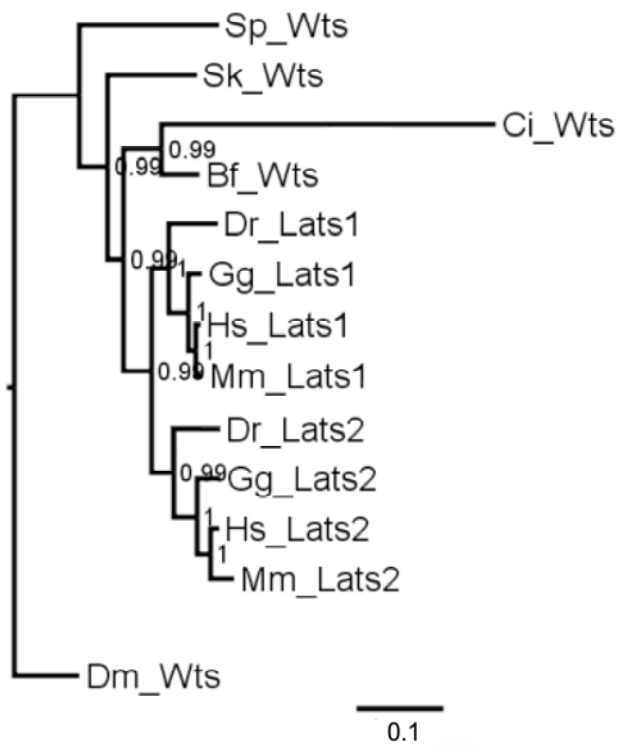
Fig. S1C. Warts/Lats Bayesian tree
