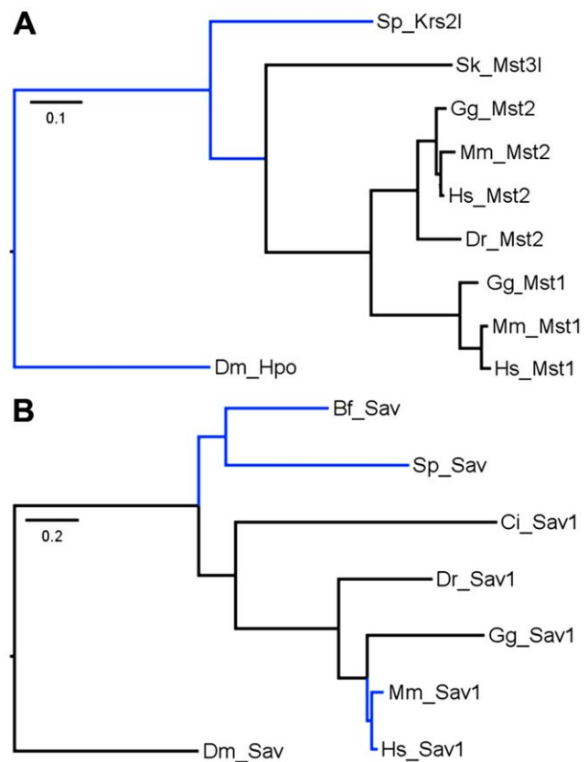
Figure 2. Hippo/Mst and Salvador Maximum Likelihood trees. Trees rooted with D. melanogaster are shown. Branches considered statistically weak (aLRT values < 0.70) are colored in blue. Branch lengths are drawn to scale and correspond to the average number of amino acid changes per site as indicated by the scale bar. A) Hippo/Mst vertebrate topology matches the species tree. Among invertebrates the hemichordate strongly clusters with vertebrates while the echinoderm is an outlier. The overall Hippo/Mst tree matches the species tree. The Bayesian tree (Figure S1A) shows one difference - the hemichordate moves out of the strong cluster with vertebrates to become an outlier like the echinoderm. B) Salvador vertebrate topology matches the species tree. Among invertebrates the urochordate clusters tightly with vertebrates while the echinoderm and cephalochordate are outliers. The overall Salvador tree matches the species tree. The Bayesian tree (Figure S1B) shows one difference - the cephalochordate clusters outside the urochordate and vertebrate cluster with confidence. doi:10.1371/journal.pone.0051599.g002
