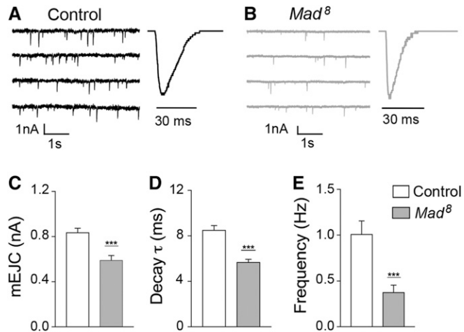
Figure 7 Electrophysiological deficits at Mad 8 NMJs. (A and B) Representative traces of spontaneous junction currents (left) and average mEJC traces (right) recorded at 0.5 mM \text{Ca}^{2+} from muscle 6, segment A3, of control (A) and Mad 8 NMJs (B). Summary graphs showing the mean amplitude (C), decay time constant (D) and mean frequency (E) of mEJCs. Error bars indicate SEM. *** P < 0.0001.
