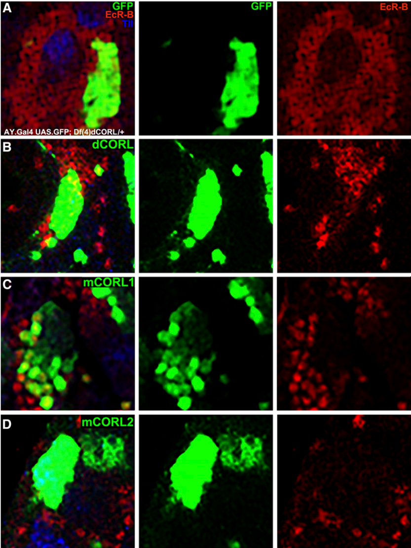
Figure 4 Repression of EcR-B1 in the MB of wild type by mCORL2/dCORL not mCORL1. High magnification dorsal view with anterior up of mushroom body neurons in the brains of wild type siblings ( Df(4)dCORL/+ ) of the mutants shown in Fig. 3. An image of a single slice is shown from left to right with genotype and clone location determined as in Fig. 3. A) A clone expressing AY.Gal4 UAS.GFP on II alone. EcR-B1 is unaffected ( n = 6). B) A clone expressing AY.Gal4 UAS.GFP on II and UAS.dCORL on III. EcR-B1 is reduced in the clone ( n = 4). C) A clone expressing AY.Gal4 UAS.GFP on II and UAS.mCORL1 on III. Where EcR-B1 overlaps the clone it is largely unaffected ( n = 8). D) A clone expressing AY.Gal4 UAS.GFP on II and UAS.mCORL2 on III. EcR-B1 is reduced in the clone, a phenotype of dCORL ( n = 15). Numerical data in Table 1.
