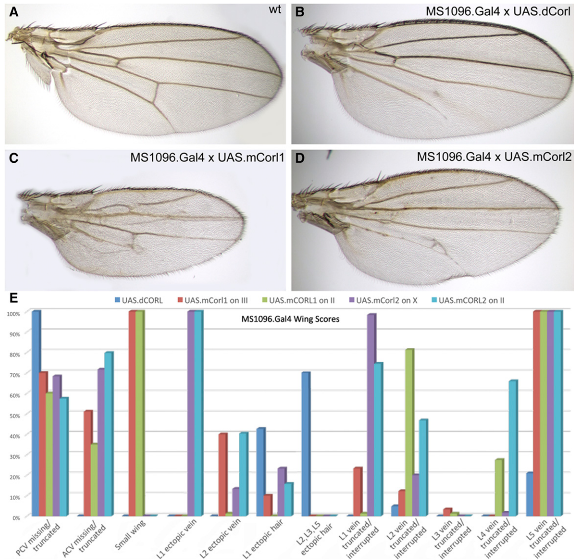
Figure 2 mCORL1 and mCORL2 are not clearly distinguished from dCORL in wing assays. A) Wild type adult female wing. B) UAS.dCORL wing is normal size with 4 ectopic margin bristles on longitudinal vein1, missing posterior crossvein and truncated longitudinal vein5. C) UAS.mCORL1 wing is on average 40% smaller than wild type, has an interrupted longitudinal vein2, missing anterior crossvein and truncated longitudinal vein5. D) UAS.mCORL2 wing with a bifurcated longitudinal vein4, missing anterior crossvein and delta at the posterior crossvein. E) Graph of all phenotypes scored for dCORL and two insertions each of mCORL1 and mCORL2. Of 12 phenotypes, four are in common, four are found only in mCORL1 and mCORL2 and there is one each unique to mCORL1 and mCORL2. Numerical data in Table S1.
