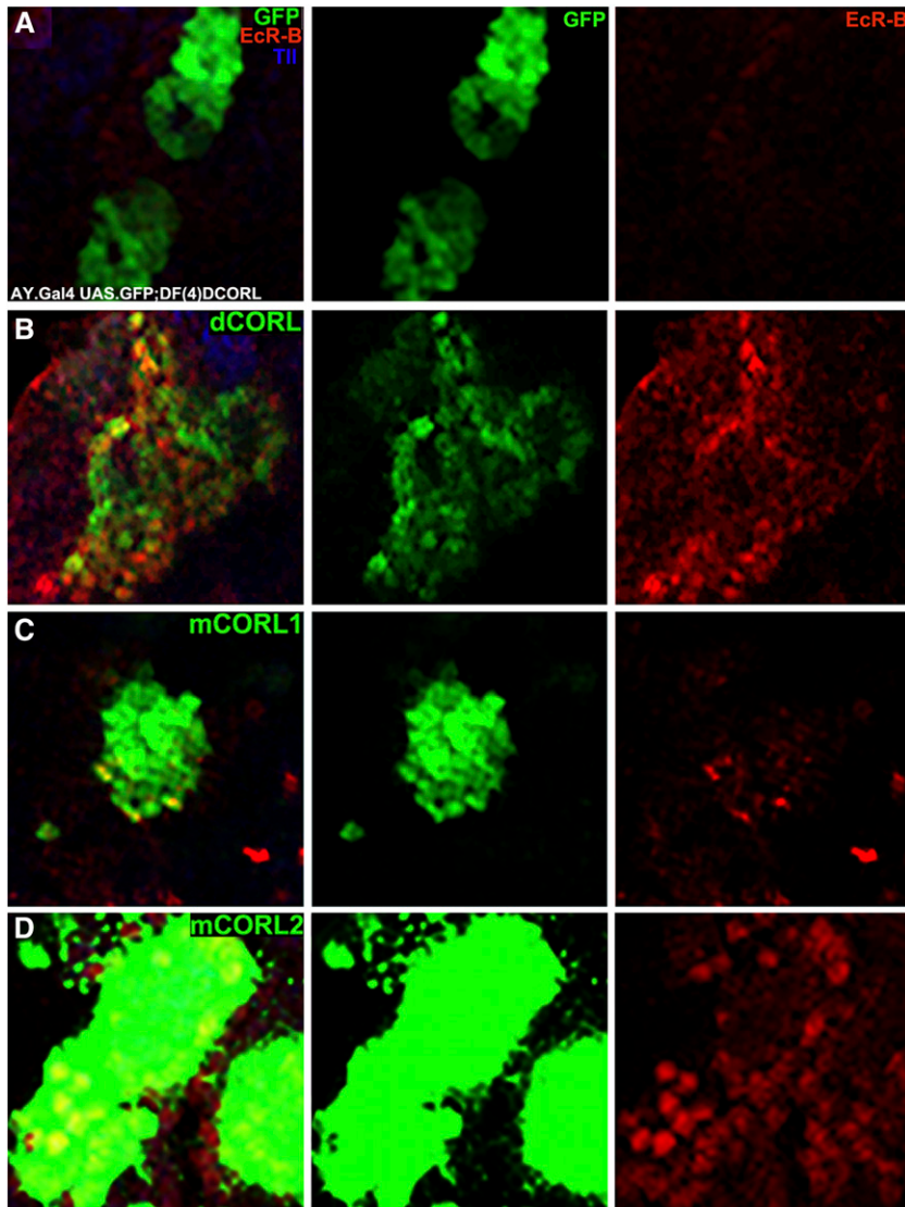
Figure 3 Rescue of EcR-B1 in the MB of dCORL mutants by mCORL2/dCORL not mCORL1. High magnification dorsal view of mushroom body neurons in Df(4)dCORL brains with anterior up. An image of a single slice is shown from left to right as three color (includes Tailless in blue), green alone (GFP), and red alone (EcR-B1). Genotype determined by reference to the sister brain lobe and clone location by reference to Tailless in MB neuroblasts not affected in Df(4)dCORL . A) A clone expressing AY.Gal4 UAS.GFP on II alone. EcR-B1 is absent ( n = 6 ). B) A clone expressing AY.Gal4 UAS.GFP on II and UAS.dCORL on III. EcR-B1 is rescued ( n = 8 ). C) A clone expressing AY.Gal4 UAS.GFP on II and UAS.mCORL1 on III. EcR-B1 expression is faint ( n = 12 ). D) A clone expressing AY.Gal4 UAS.GFP on II and UAS.mCORL2 on III. EcR-B1 is rescued, a phenocopy of dCORL ( n = 8 ). Numerical data in Table 1.
