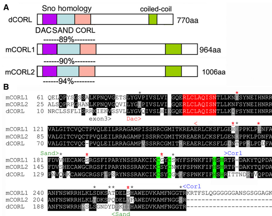
Figure 1 mCORL1 and mCORL2 are equidistant from dCORL in the Sno homology domain. A) Schematic of CORL proteins from fly and mouse with the locations of five named domains shown. Amino acid similarity in the Sno homology domain (Smad binding; 195 residues) between dCORL and mCORL1 is shown above mCORL1, between dCORL and mCORL2 above mCORL2 and between mCORL1 and mCORL2 below mCORL2. Similarity is the sum of identical residues and conservative substitutions where both amino acids share biochemical properties: D/E, K/R/H, N/Q, S/T, I/L/V, F/W/Y, A/G (Smith and Smith 1990). B) Sno homology domain alignment. An amino acid is shaded if the residue is identical (black) or similar (gray) in two or three proteins. The APC recognition site is red and Cys2-His2 zinc finger in green. The Dac, Sand and CORL domains are shown with arrowheads. Fourteen amino acids different between mCORL1 and mCORL2 are indicated by *, a red * indicates 6 positions where dCORL and mCORL2 both differ from mCORL1 and red ± indicates 4 positions where mCORL1 has a biochemically distinct amino acid from both dCORL and mCORL2.
